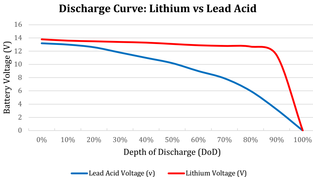
Figure 6 – Volt Curve Lead Acid vs Lithium
